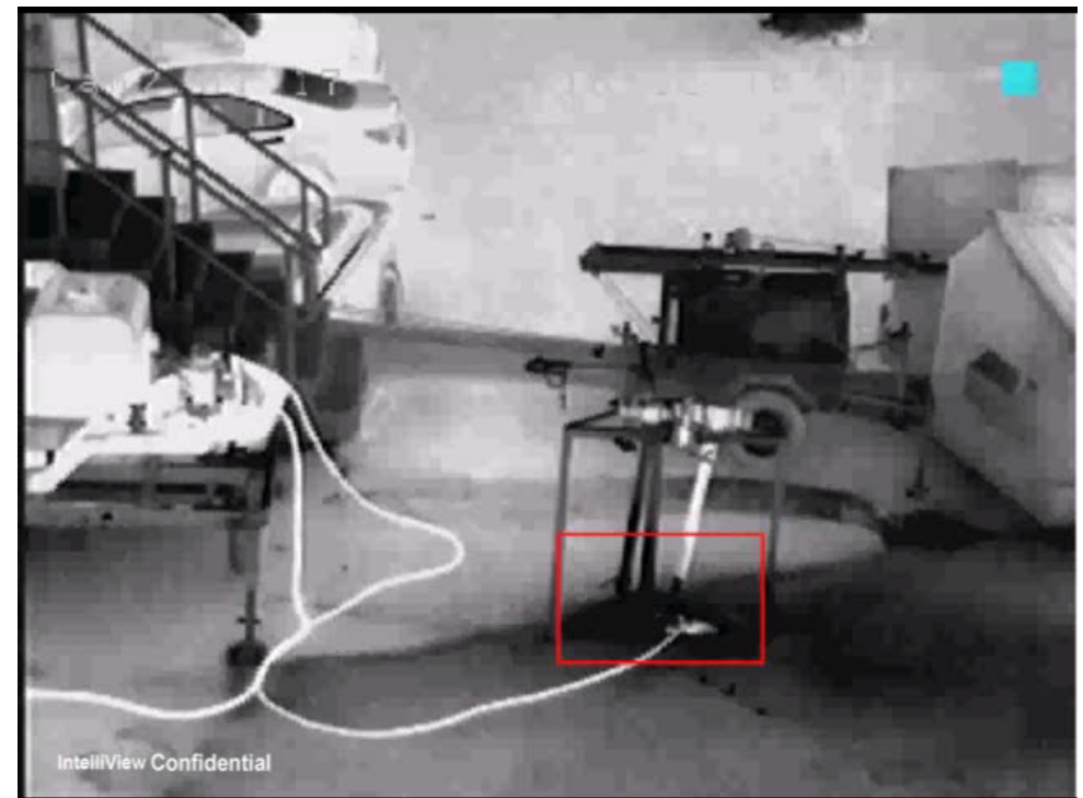
Small Flange drip Leak at 50 feet
